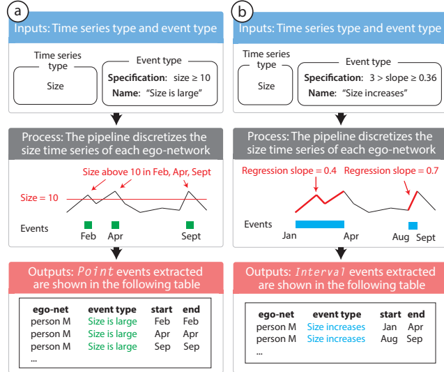
Figure 4: The inputs, process and outputs for extracting events from dynamic ego-networks. (a) Point events are created when the event type's specification is a range of values (e.g., \text{size} \geq 10 ). (b) Interval events are created when the specification is a range of slopes (e.g., 3 > \text{slope} \geq 0.36 ).
