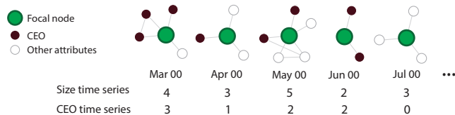
Figure 2: A dynamic ego-network in the Enron email network. It is represented as multiple time series (e.g., size and CEO) in Segue.
